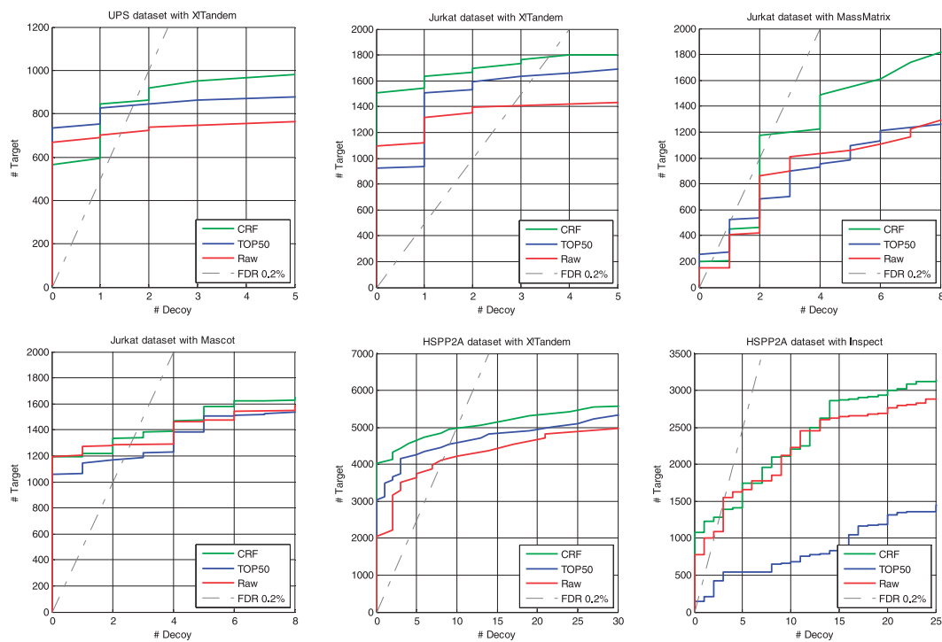
Fig. 5. ROC analysis of the spectrum annotation results of the raw data and the CRF and Top50 filtered Jurkat, HSP2A and the UPS datasets, obtained with X!Tandem, Mascot, InsPecT and MassMatrix. These plots show independent improvements by the CRF filter on various search engines
